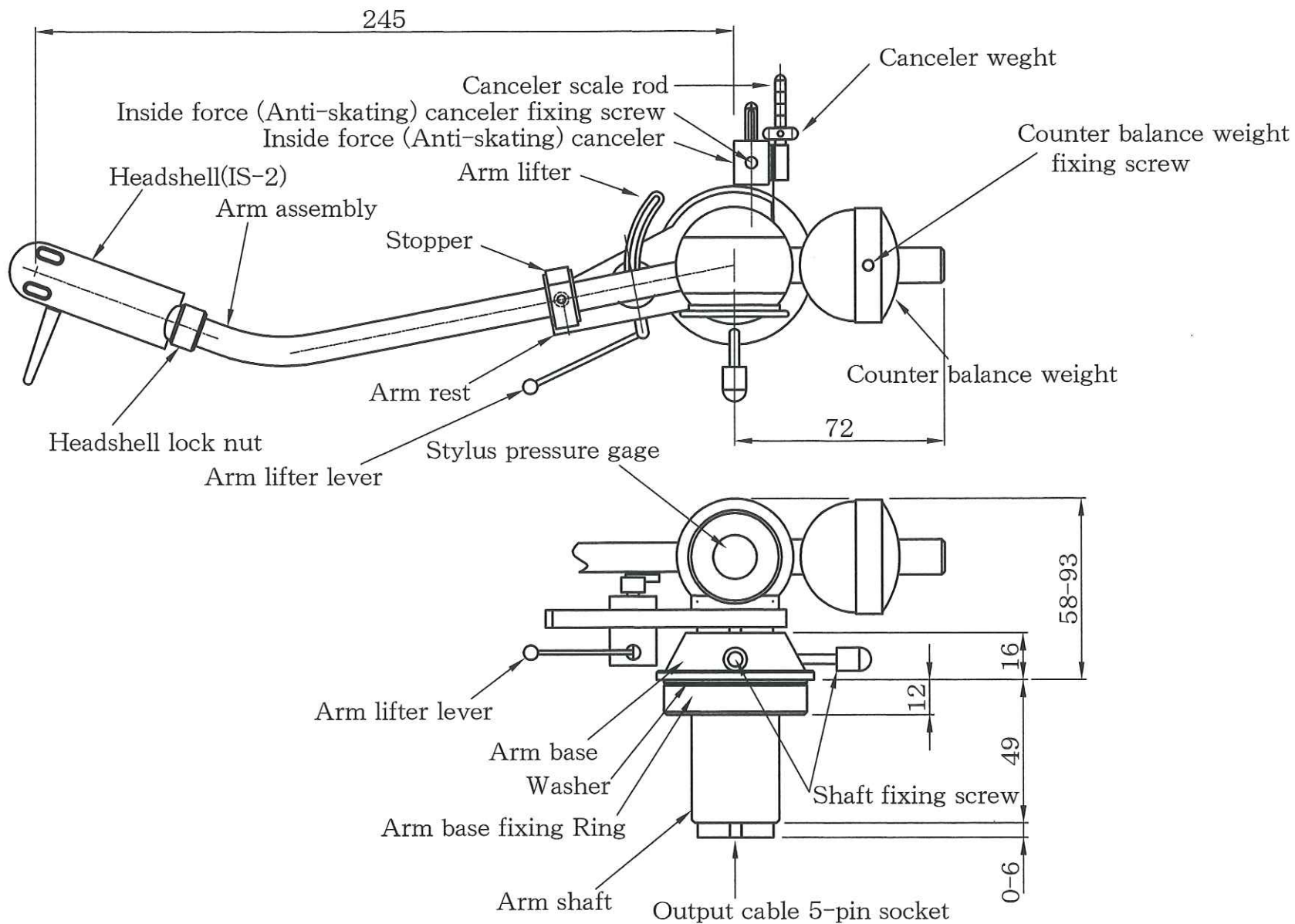
Dynamic Balance Tonearm. Model : IT-345
